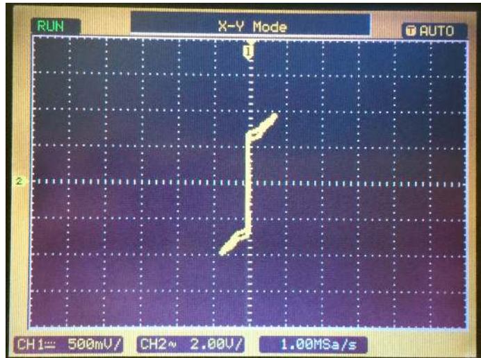
Figure 7: The DC Josephson effect. Vertical scale is 0.500 mA/div, and horizontal scale is 2.00 V/div. See Section 5.1 for a recreated I-V plot, which uses actual data points extracted with the Josephson junction.vi program made available by the 111B lab. Image captured using iPhone 6S Plus.
