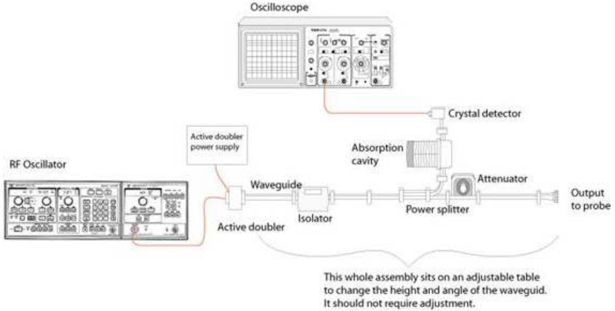
Figure 8: Relevant equipment for the AC effect portion of the experiment. Image sourced from [7].
