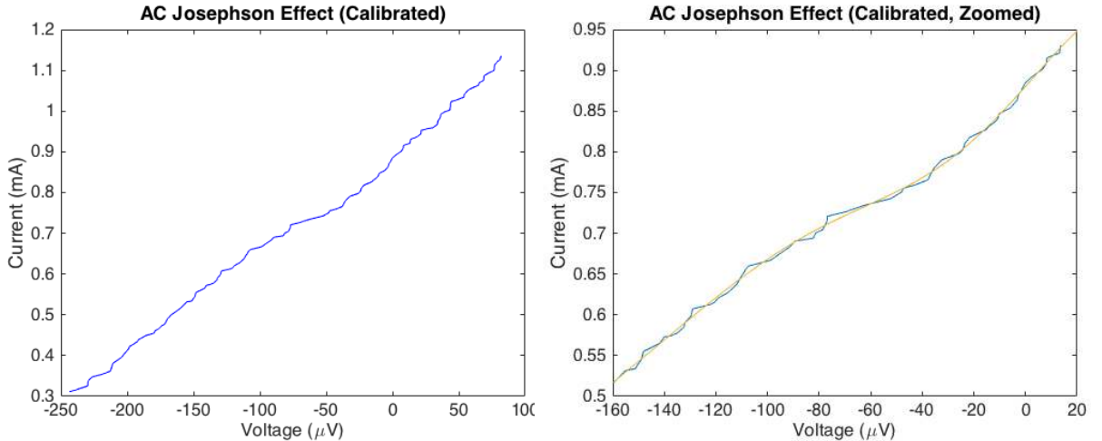
(a) Voltage-calibrated plot of the AC effect I-V (b) Voltage-calibrated plot, zoomed in on the “step” characteristic. Data taken using the Josephson junction.vi program provided by the 111B lab. and fitted with CurveFit.m script provided by the 111B lab.
